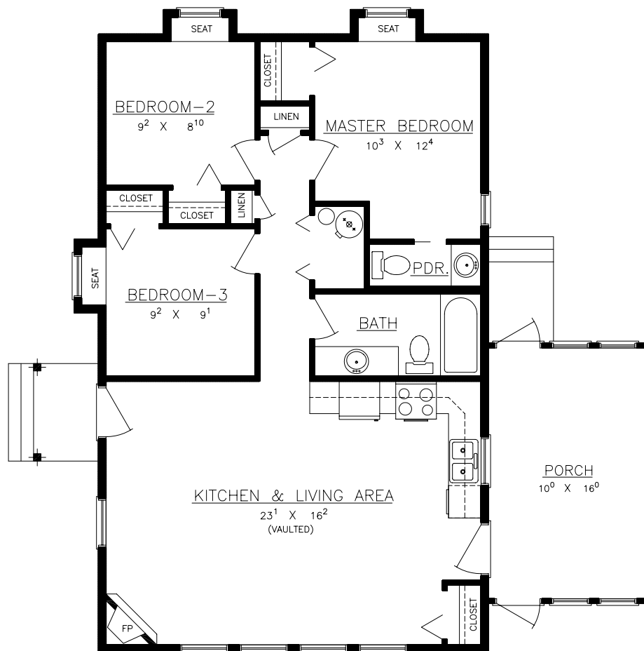
FLOOR PLAN
